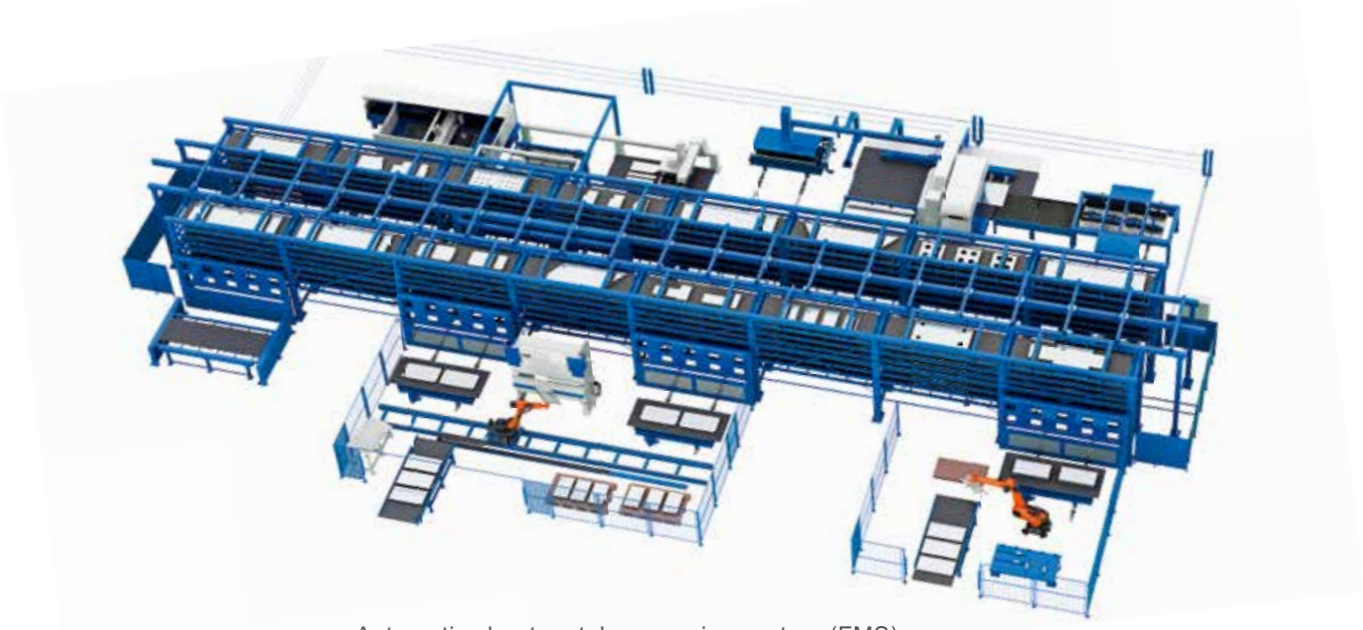
Automatic sheet metal processing system (FMS)
