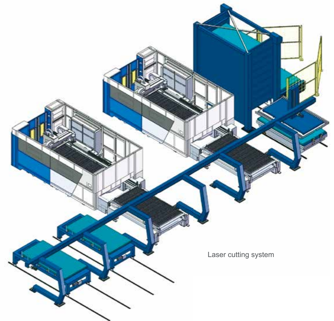
Laser Cutting Unit - Programs II
